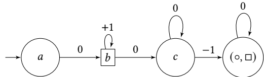
Figure 2: A two-player game with a solution.
